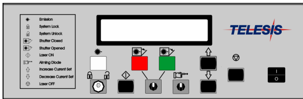
XP1 Laser Controller
