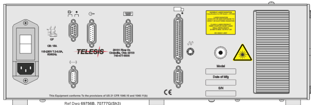
E1015 Laser Controller Back Panel – External Computer
